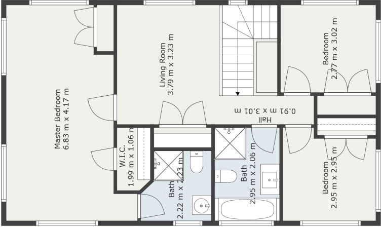
Floor 2
